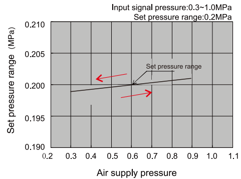
EPR3000 Pressure characteristics
